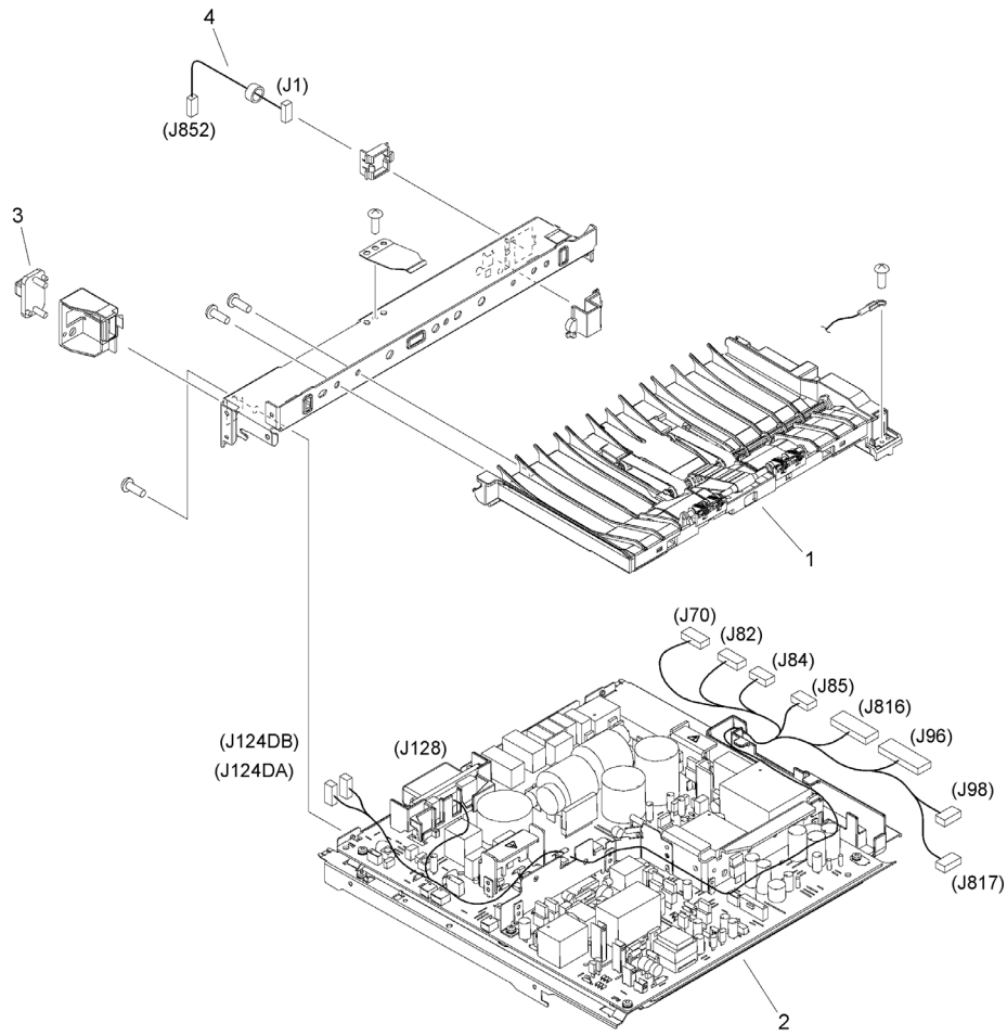
Figure 110A POWER SUPPLY ASS'Y (100V, 120V)
