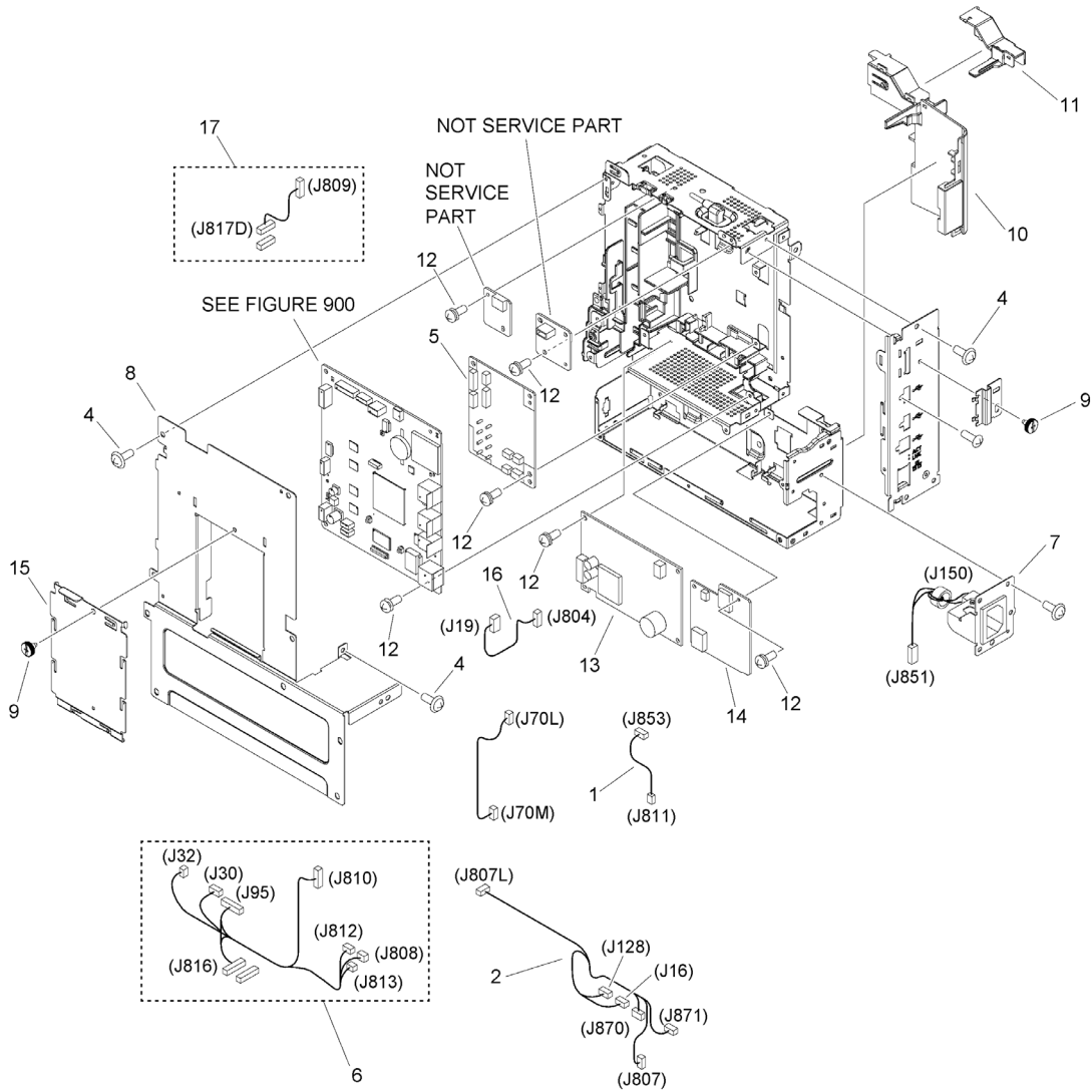
Figure 104B INTERNAL COMPONENTS 4
