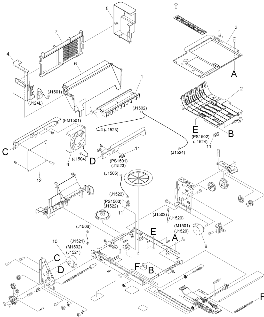
Figure S10 DUPLEXING UNIT
