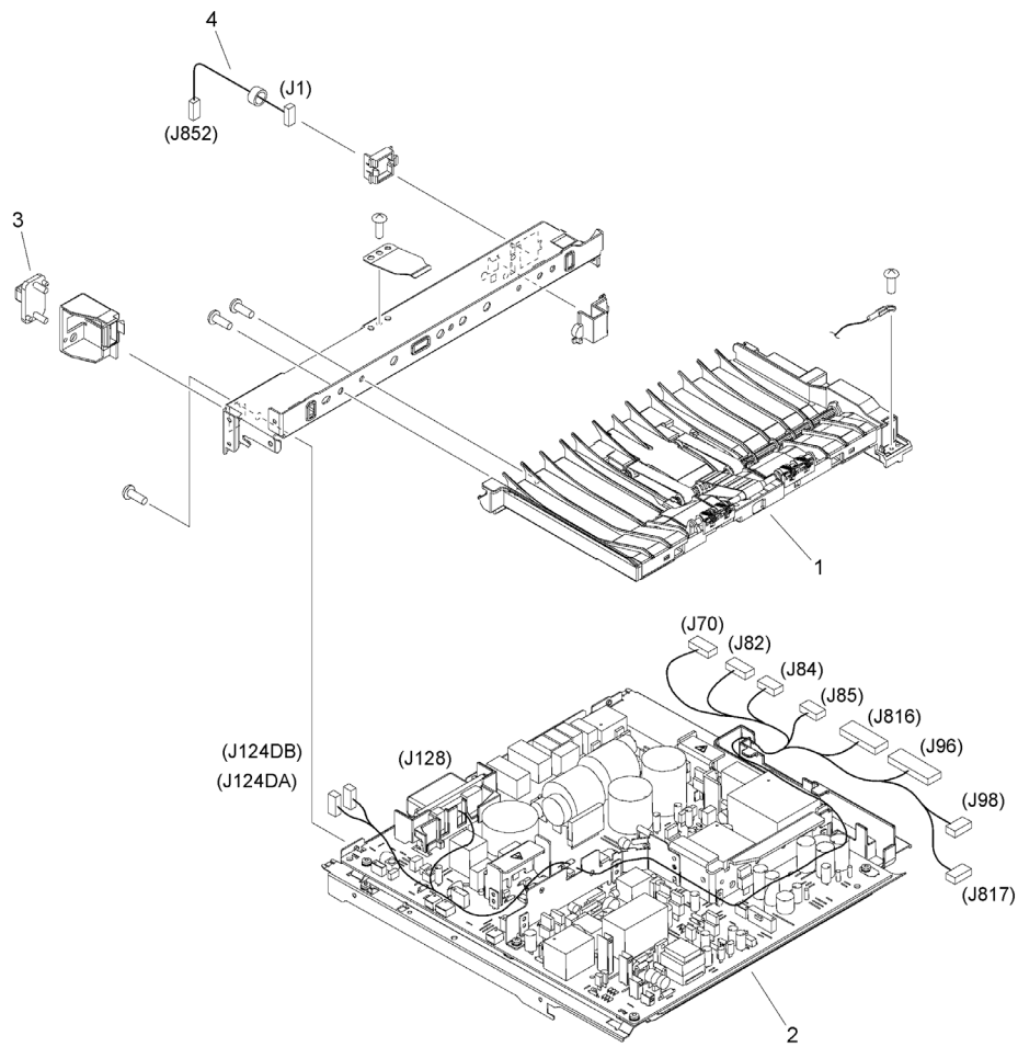
Figure 110B POWER SUPPLY ASS'Y (230V)
