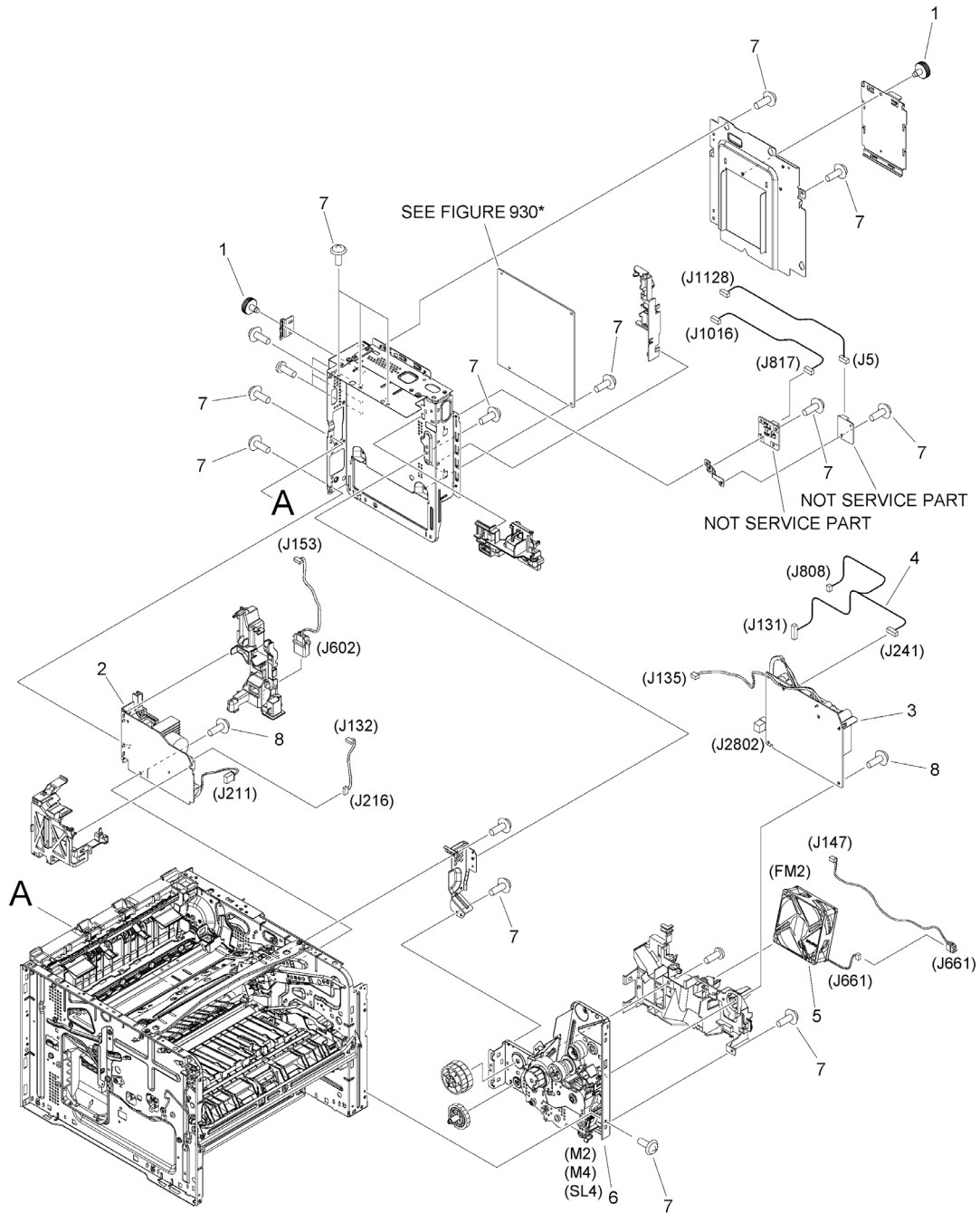
Figure 104A INTERNAL COMPONENTS 4 (LBP312i, LBP312dn)
