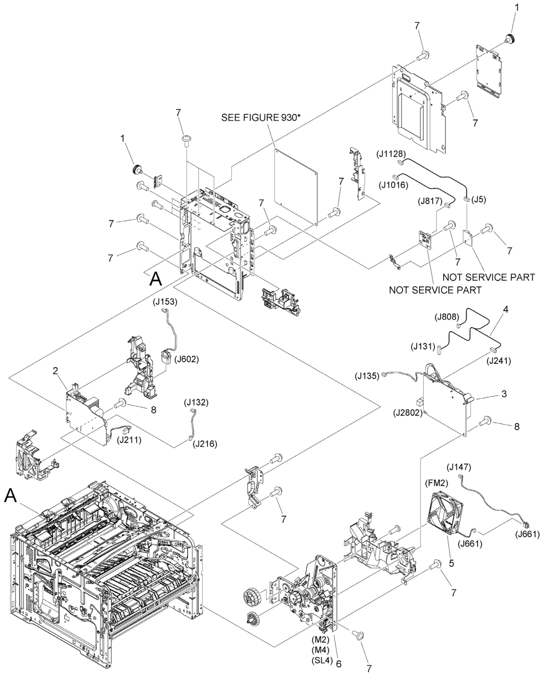
Figure 104B INTERNAL COMPONENTS 4 (LBP312x, LBP311x, LBP310x)
